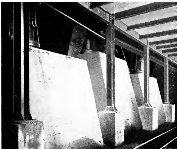
Fig. 157. View showing Several Jolt-Ramming Moulding Machine Foundations with Piers built on the Basement Floor.
